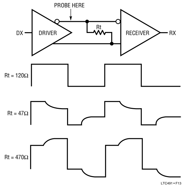
Figure 13. Termination Effects
